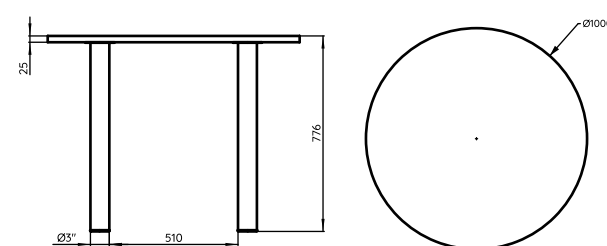
MESA CLÁSICA Ø1000MM - PATA Ø3"
