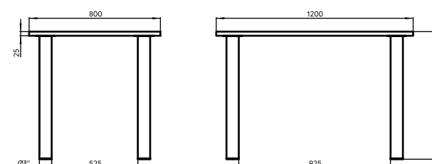
MESA CLÁSICA 1200X800MM - PATA Ø3"
