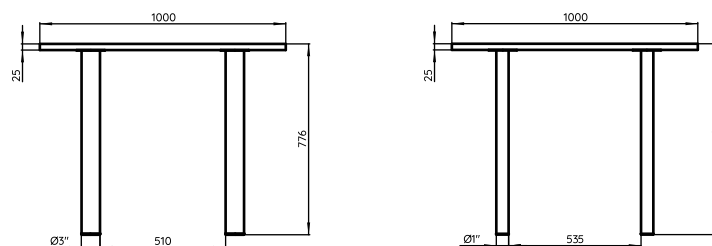
MESA CLÁSICA 1000X1000MM - PATA Ø3"
